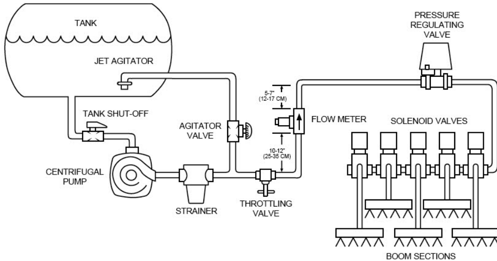
Figure 1-4: Throttling Plumbing Diagram - Pressure Based System
