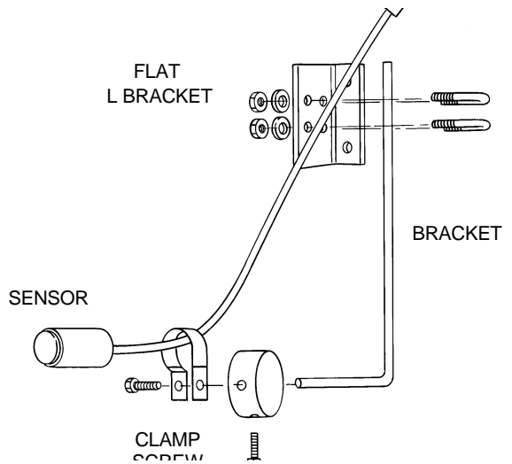
Figure 1-10: Sensor Assembly diagram showing the components and their assembly.
