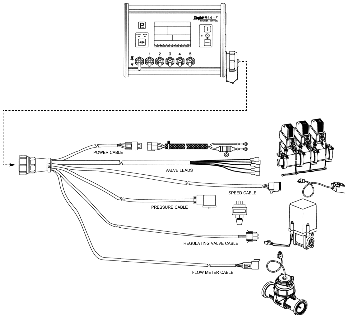
Figure 1-14: Wiring Layout
