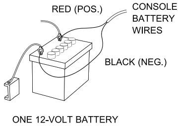
Figure 1-12: Power Connection
