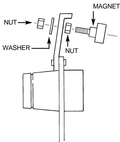
Figure 1-8: Magnet Assembly
