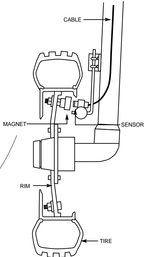
Figure 1-5: Wheel Mounting of Magnetic Speed Sensor
