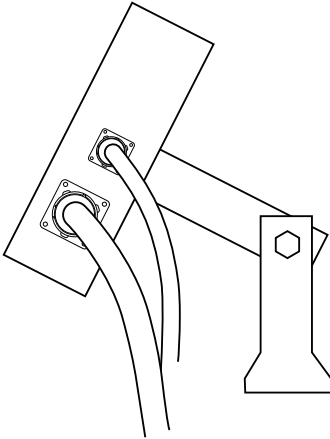
Figure 1-11: Brackets Provide Angle Adjustment
