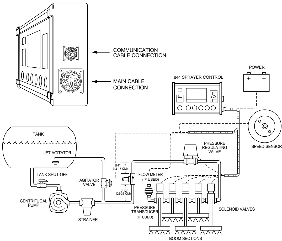
Figure 1-13: Wiring Diagram
