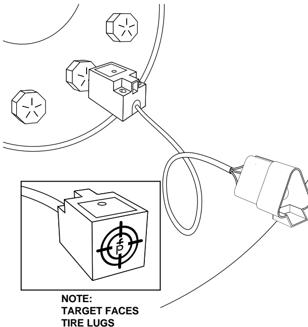
Figure 1-6: Wheel Mounting of Speed Sensor
