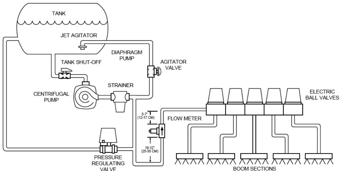
Figure 1-2: Bypass Plumbing Diagram - Flow Based System
