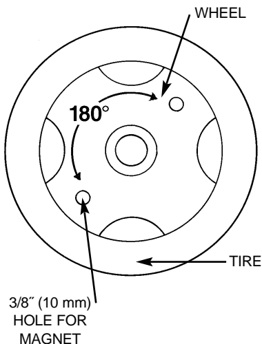
Figure 1-7: Magnet Locations
